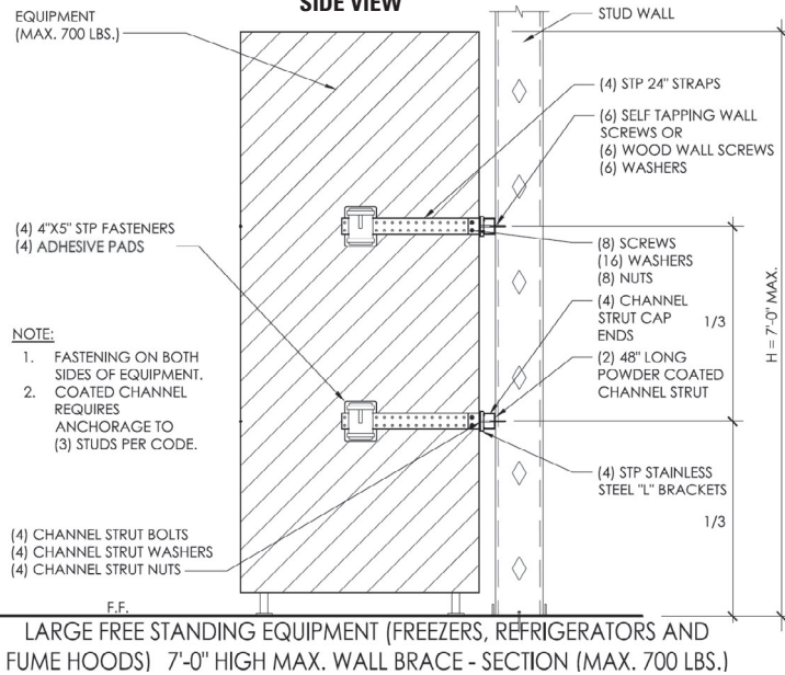
SIDE VIEW
